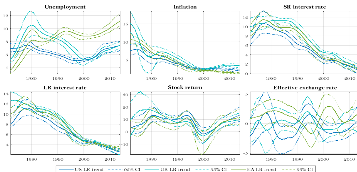
Figure 3: Long-run trends
